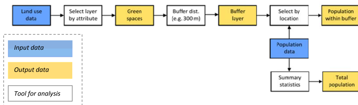
Fig. 4.1 GIS flow chart for the basic method (ArcGIS)
